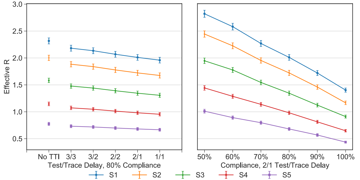
Figure 5: Impact of testing/tracing delays and compliance on \mathcal{R} , for the test-based TTI strategy.
