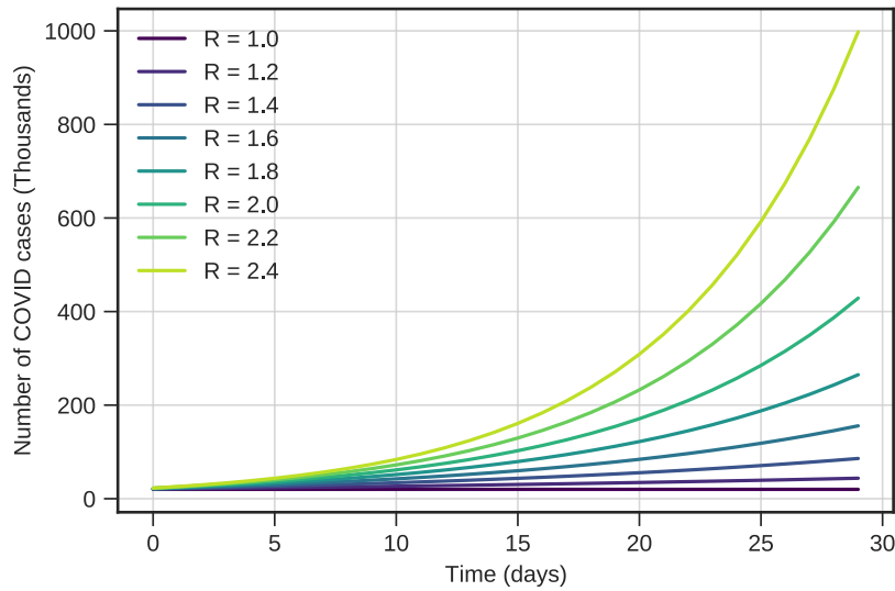
Figure 18: Relationship between expected number of new cases and \mathcal{R} over time.
