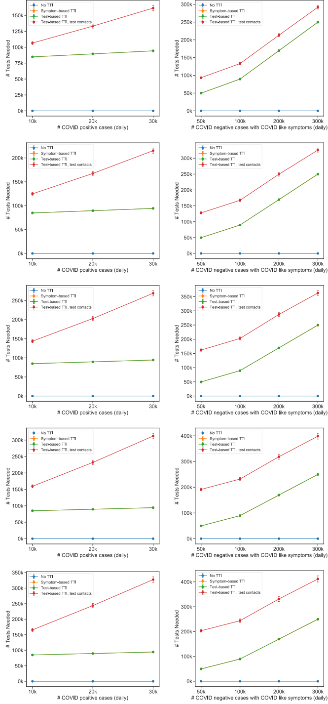
Figure 16: Left: Effect of varying number of new COVID cases per day on the number of tests needed. Right: Effect of varying the number of COVID negative cases with COVID-like symptoms on the number of tests needed. The number of tests required for symptom-based TTI is the same as for test-based TTI, as we assume all primary cases are tested. Top to Bottom: S5 down to S1.
